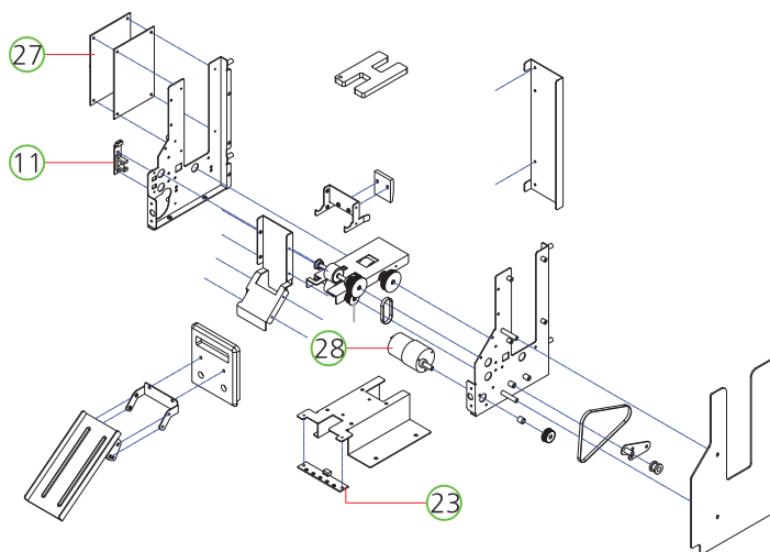
- MEDAL EV HOPPER(FONT)
