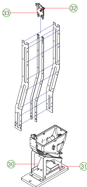
- MEDAL EV HOPPER(FONT)
