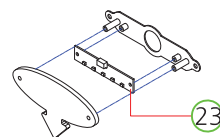
- GAUNTLET DECO PART
