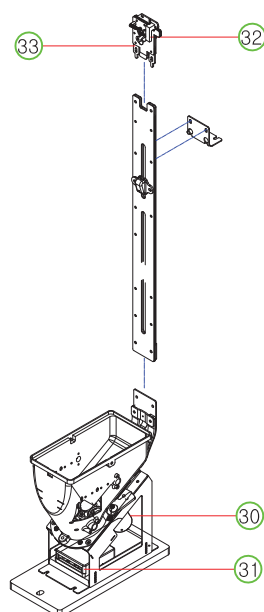
- MEDAL EV HOPPER(REAR)
