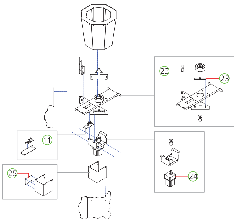
- BIG WHEEL PART
